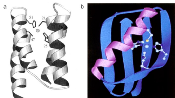
Figure 5. (a) Model of \text{Z}\alpha_4 . The side chains (clockwise from top right) are Cys21, His25, Cys47, and His51. Panel a was reproduced from ref 70. Copyright 1995 American Chemical Society. (b) Model of the metal-binding site in the B1 domain of streptococcal protein G. The ribbon diagram is specifically of \text{Z}\beta_1\text{M} . The side chains around the metal-binding site are His16, His18, His30, and Cys33. Panel b was reproduced from ref 76. Copyright 1995 Nature Publishing Group.
