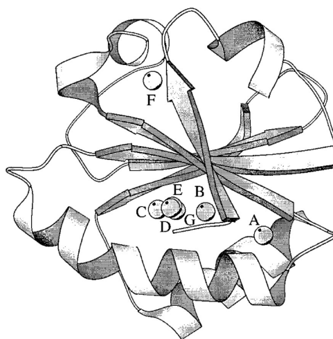
Figure 6. Distribution of the designed \text{Cys}_2\text{His}_2 sites in thioredoxin (letters identify each design). This figure was reproduced ref 84. Copyright 1998 American Chemical Society.
